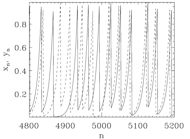
Fig. 1. Time series of Bernoulli-like maps ( x_n solid line, y_n dashed line) for a = 1.1 , \gamma = 0.15 , M = 5 . The coupling is set on at n = 5000 , leading to anticipated synchronization.
