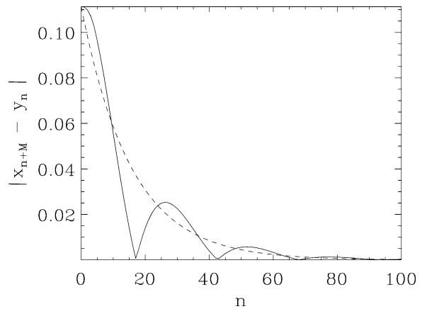
Fig. 3. Transient decay of |x_{n+M} - y_n| for a = 1.1 , M = 5 and \gamma = 0.15 . The solid line indicates the value of |x_{n+M} - y_n| and the dashed line indicates the value of |x_M - y_0| \exp(-n/\tau) with \tau = -1/\ln|z_1| \sim 15.55 as explained in the text.
