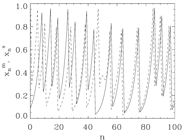
Fig. 4. Time series of the 2D Baker map ( x_n^m solid line, x_n^s dashed line) for a = 1.333 , b = 0.777 , \gamma = 0.7 , and M = 1 . The coupling is set on at n = 30 , leading to anticipated synchronization.
