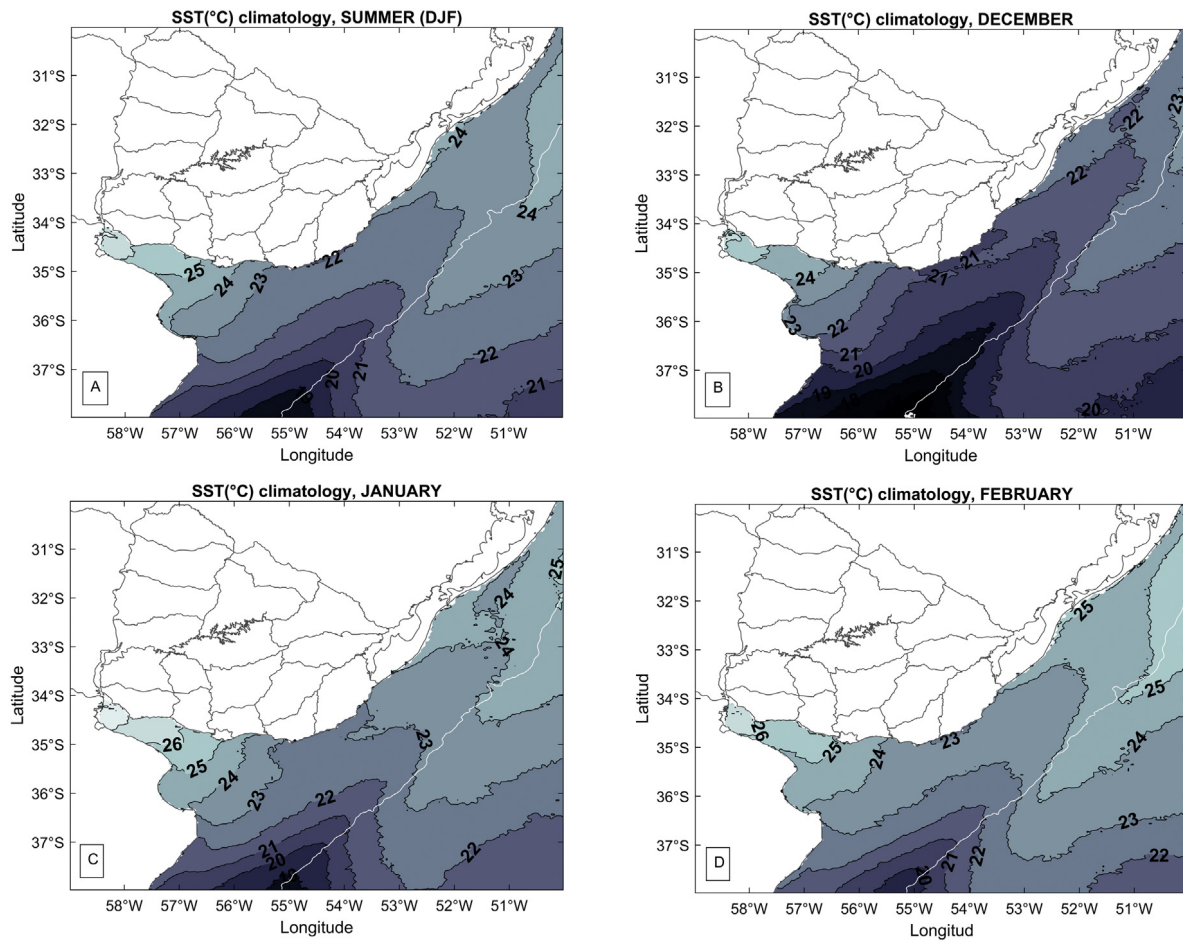
Fig. 2. (a) Summer (DJF) and (b, c, d) monthly climatology of sea surface temperature (°C); the white line is the 200 m isobath and the numbers in contour are sea surface temperature (°C) values.
