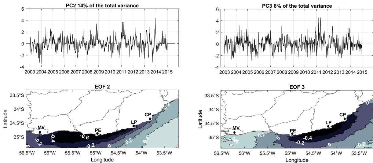
Fig. 3. Modes of variability of sea surface temperature anomaly in the domain considered. Empirical orthogonal function (EOFs) and Principal component time series (PCs) which represents 14% and 6% of the total variance. Coastal localities are indicated with black dots: Montevideo (MV), Punta del Este (PE), La Paloma (LP) and Cabo Polonio (CP).
