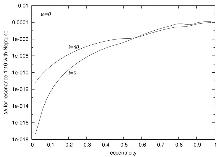
Figure 6: Typical strength for all interior and exterior resonances of order q \geq 2 . At low eccentricities the resonances are stronger for high inclination orbits and at high eccentricities the inclination do not affect substantially the resonance's strength. This particular plot corresponds to resonance 1:10 with Neptune.
