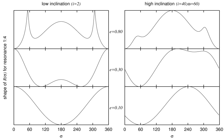
Figure 1: General behavior of R(\sigma) for 1:n resonances for three values of e and two values of i . The lower plot correspond to e < e_a < e_c (see text), at left three plots for low inclination orbits and at right for high inclination orbits. Trojans also exhibit this behavior except the lower panel because for trojans e_c = e_a = 0 . Stable librations are possible at minima of R(\sigma) but the asymmetric librations also allow HS trajectories wrapping both asymmetric libration islands, so \sigma seems to oscillate around 180^\circ with very high amplitude. For high inclination orbits the shape of R(\sigma) is completely distorted and shallow minima can appear besides of a well defined one.
