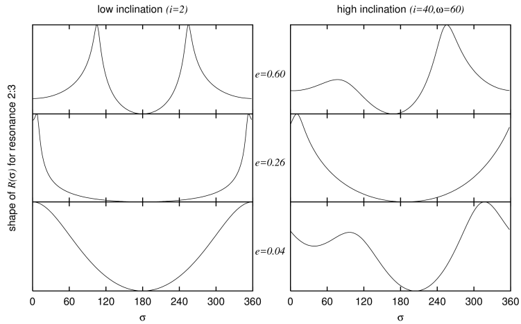
Figure 4: General behavior of R(\sigma) for three values of e and two values of i for even order interior resonances and all exterior resonances except 1:n . The lower plot corresponds to e < e_c . Compare this figure with Fig. 2.
