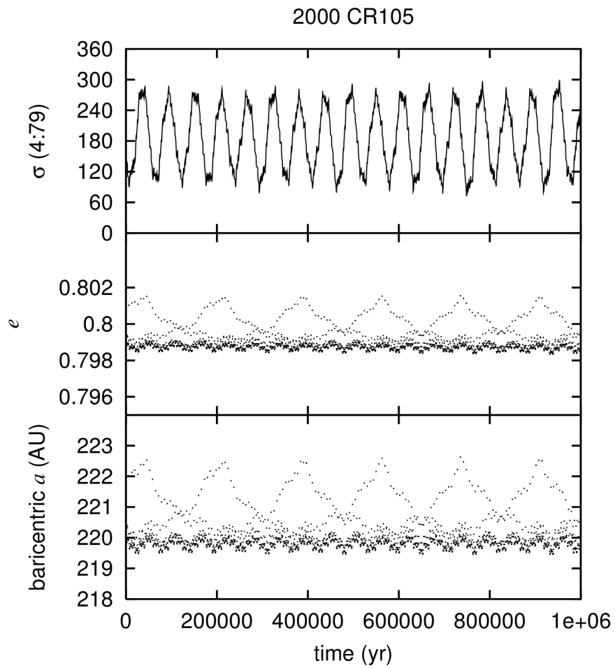
Figure 8: Resonant motion of 2000 CR105 inside the resonance 4:79N according to nominal orbit from ASTORB. The critical angle is \sigma = -4\lambda_N + 79\lambda - 75\varpi .
