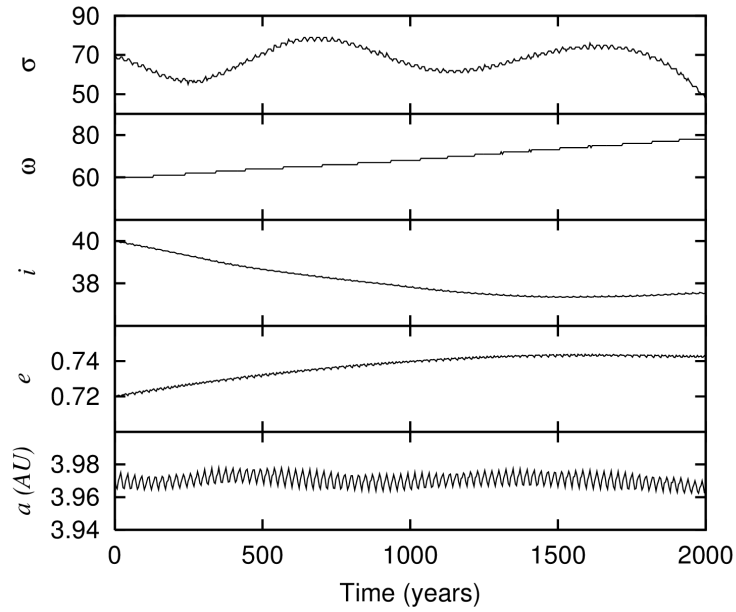
Figure 3: Verification of the existence of the stable equilibrium point at \sigma \sim 70^\circ deduced from Fig. 2. Numerical integration of an hypothetical particle at resonance 3:2 with Jupiter. The libration center is strongly linked to (i, \omega) . The libration period (poorly distinguished in a ) is approximately 800 years.
