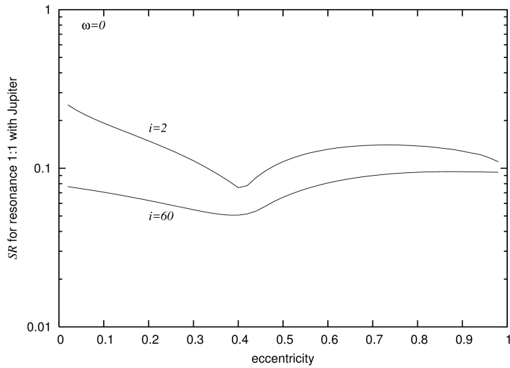
Figure 5: Typical behavior of the strength function SR for trojans and all first order resonances ( q \leq 1 ). Low inclination orbits are in general something stronger than high inclination orbits. This particular plot corresponds to Jupiter's trojans but all first order resonances show a similar behavior with respect to the inclination.
