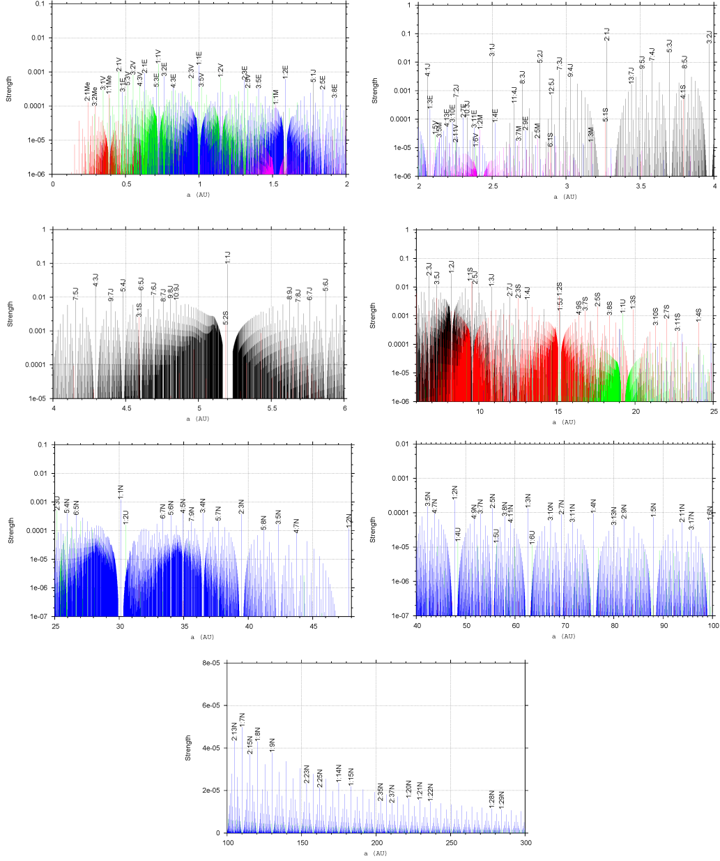
Figure 7: Atlas of MMRs in the solar System verifying |p+q| < 100 and with order q < 100 calculated for different set of values ( e, i, \omega = 60^\circ ) characteristic of some populations of minor bodies. (a) Terrestrial planets' region. The resonance's strength is calculated for typical NEAs' orbits ( e = 0.46, i = 15^\circ ). Resonances with Venus and Earth dominate. Between 1.5 and 2 AU resonances 1:2E, 2:5E and 3:8E are strong and isolated. (b) Asteroids' region. The resonance's strength is calculated as in (a). Between 2 and 2.5 AU several high order resonances with Venus, Earth and Mars compete with resonances due to Jupiter. Note the behavior of the strength of the family of resonances near 2:1J slightly perturbed by 5:1S and the isolation of resonance 3:2J. (c) Jupiter's region. The resonance's strength is calculated as in (a). The pattern is due to Jupiter which dominate this region. Jupiter's trojans are perturbed by 5:2S. (d) Centaurs' region. The resonance's strength is calculated for orbits with e = 0.46, \vartheta = 32^\circ . Note the superposition of resonances with Jupiter and Saturn. (e) Neptune's and TNOs' region. The resonance's strength is calculated for orbits with e = 0.2, i = 10^\circ . The pattern of the resonances in this region is imposed by Neptune. Neptune's trojans could be affected by 1:2U. (f) Scattered Disk Objects' region. The resonance's strength is calculated for SDOs evolving with q = 32 AU and assuming i = 20^\circ . (g) The farthest regions of the Solar System. The resonance's strength is calculated as in (f). In this plot the scale in strength is linear. Resonances 1:n with Neptune dominate.
