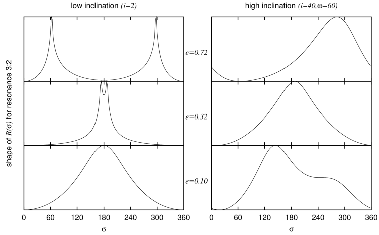
Figure 2: General behavior of R(\sigma) for all odd order interior resonances for three values of e and two values of i . The lower plot corresponds to e < e_c . See Fig. 4 for comparison. In analogy to Fig. 1, for high inclination orbits the shape of R(\sigma) is completely distorted. The equilibrium point that appears in the top right plot at \sigma \sim 70^\circ is verified in Fig. 3.
