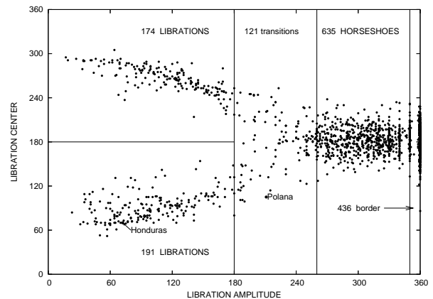
Fig. 1. The resonant population according to the firsts 10.000 years from present. The libration period is of the order of some 10^3 years. Polana with a diameter of 55 kms is the biggest asteroid.
